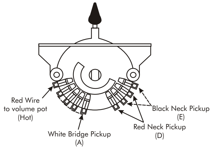
"Hot Side" Wafer Layout
